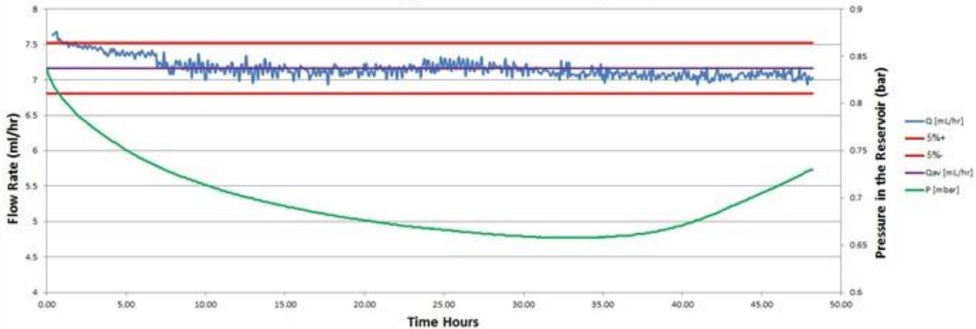
Flow Rate monitoring, SmartBlock 400ml, 7ml/hr
